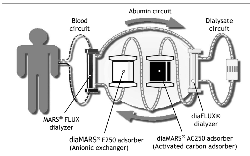
Figure 2. The Molecular Adsorbent Recirculating System (MARS) consists of a blood circuit, an albumin circuit, and a dialysate/filtrate side
