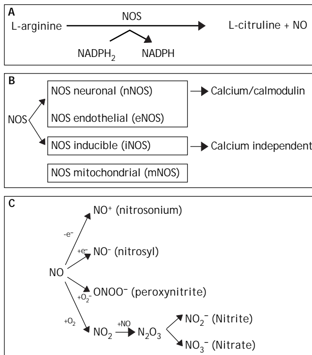
Figure 1. A. NO is synthesized endogenously by conversion of L-arginine to L-citrulline, using NADPH as an electron donor. B. The reaction is catalyzed by a family of enzymes called nitric oxide synthases (NOS). Distinct isoforms of NOS are presented. C. Under normal conditions, interaction of NO with oxygen results in the formation of the relatively inactive end products nitrite ( \text{NO}_2^- ) and nitrate ( \text{NO}_3^- ). NO can be also converted into different reactive chemical forms as nitrosonium ( \text{NO}^+ ) and nitroxyl ( \text{NO}^- ) radicals, by gaining or losing electrons, respectively. Finally, NO can combine with \text{O}_2^- (superoxide anion) to render \text{ONOO}^- (peroxynitrite).
