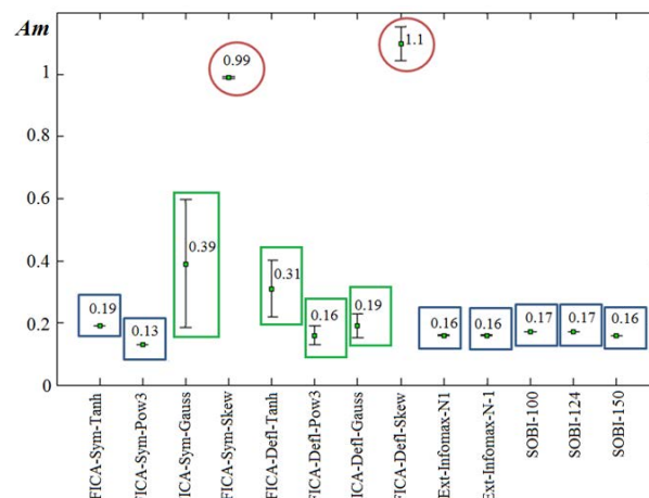
Figure 4. Mean and standard deviation of the index used to evaluate the overall quality of the separation ( Am ) achieved by each ICA configuration tested in this work.
