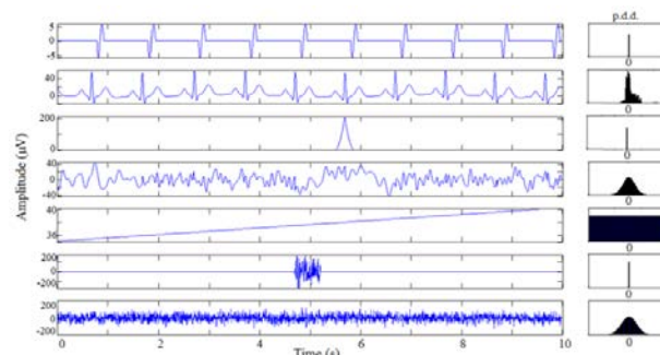
Figure 1. Ten seconds of the synthetic signals generated in this work along with their probability density distributions. From top to bottom: the LLAEP, the ECG, the eye blinking, the basal EEG, the electrode drift, the muscle activity and the electrode noise.
