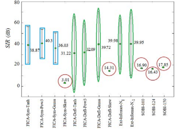
Figure 5. Mean and standard deviation of the index ( SIR ) used to evaluate the quality of the LLAEP separated by each ICA configuration tested in this work.
