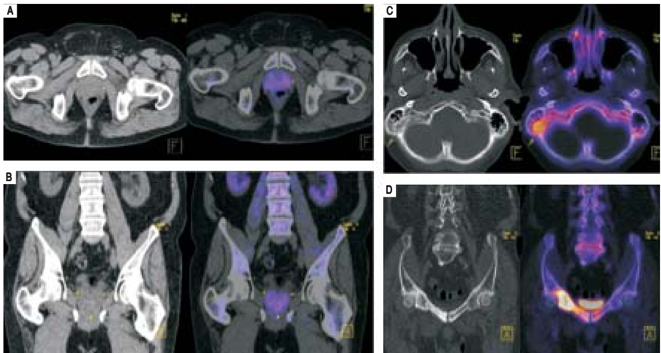
Figure 2. A-B. ^{11}\text{C} -Acetate PET-CT. 72 y.o. male with prostate cancer: High oxidative metabolism in a focal area of the prostate's left lobe. C-D. ^{18}\text{F} -NaF PET-CT. 77 y.o. male with blastic metastasis of prostate cancer: high NaF concentration in sclerotic lesions of the right mastoid bone and both superior pubic ramus, right predominant.
