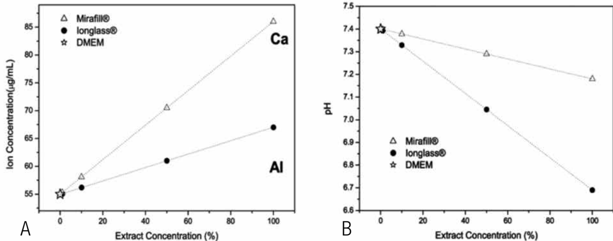
Figure 3. Extract concentration vs the amount of \text{Ca}^{2+} and \text{Al}^{3+} (A) and vs pH (B).
