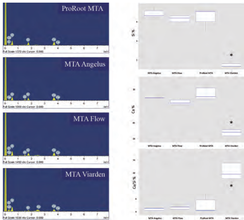
Figure 5. EDS analysis. Left column. Individual EDS spectra. Right column. Comparative box-plot show the mean (standard deviation) indicated for Ca%, Si% and Ca/Si%. (* statistical difference).
