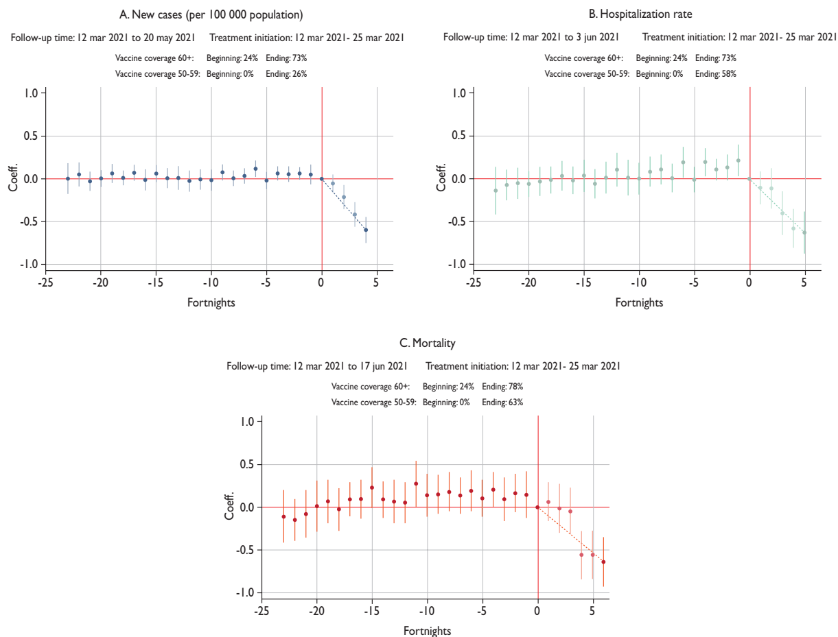
FIGURE 2. EVENT STUDY MODELS FOR CASES, HOSPITALIZATIONS, AND DEATHS PER 100 000 POPULATION, MEXICO'S EPIDEMIOLOGICAL SURVEILLANCE SYSTEM FOR VIRAL RESPIRATORY DISEASE (SISVER). 2021
